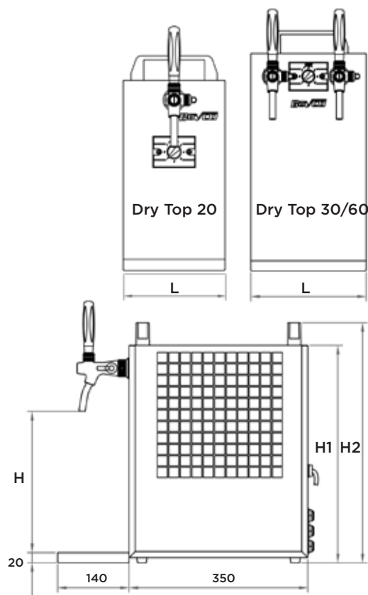
Rubinetti e raccogli gocce inclusi Taps and drip tray included
