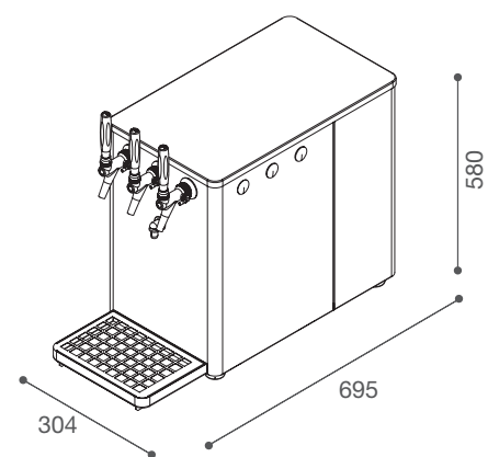
Rubinetti, kit raccorderia e serpentine non inclusi Taps, fittings and coils not included
